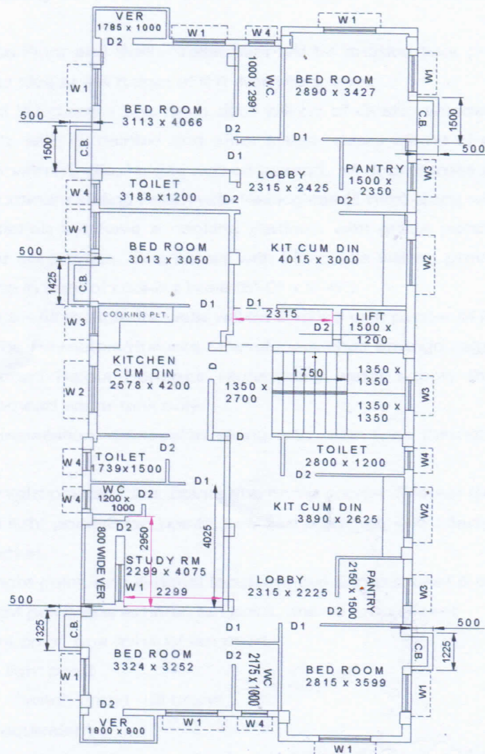
1ST ,2ND,3RD FLOOR PLAN
